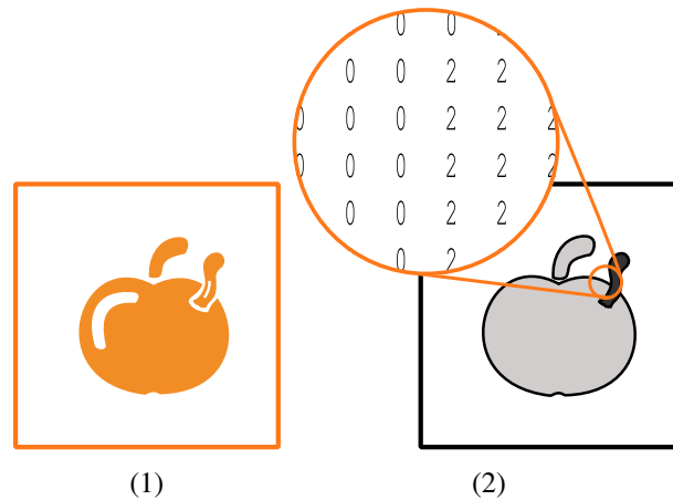
Scheme of anomaly_file_name . For visibility, gray values are used to represent numbers. (1) Input image. (2) The corresponding anomaly_file_name providing the class annotations, 0: 'ok' (white and light gray), 2: 'nok' (dark gray).
