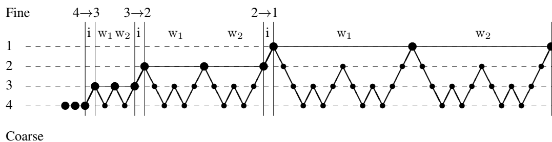
Full multigrid algorithm
