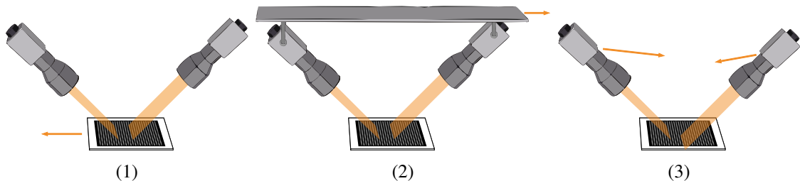
Different configurations of telecentric line scan camera setups can be distinguished: (1) Only one motion vector needs to be computed if the cameras are mounted stationary while the object is moved linearly, (2) or if the cameras are moved across the object while mounted rigidly to each other. (3) Alternatively, if the cameras are moved independently from each other, a motion vector is determined for each camera.
