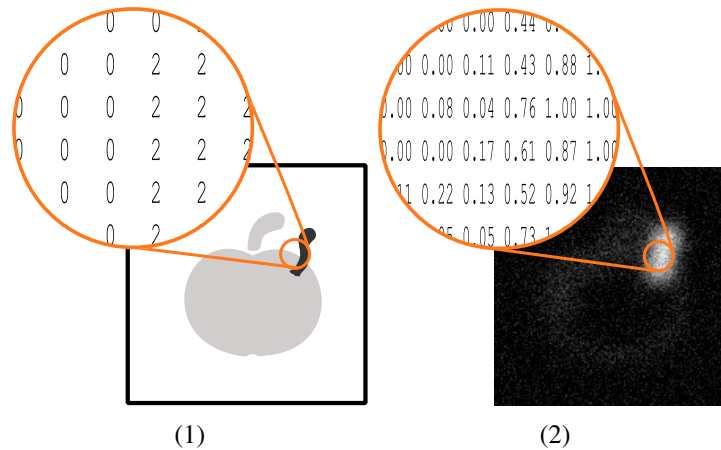
Scheme of anomaly_image . For visualization purpose, gray values are used to represent numbers. (1) The anomaly_file_name providing the class annotations, 0: 'ok' (white and light gray), 2: 'nok' (dark gray) (2) The corresponding anomaly_image .
