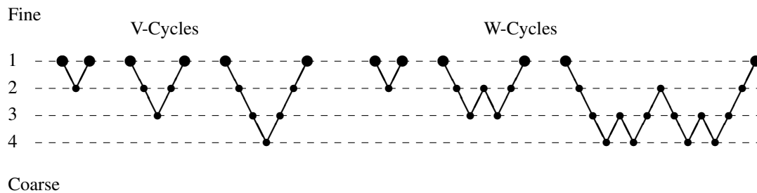
Bidirectional multigrid algorithm
