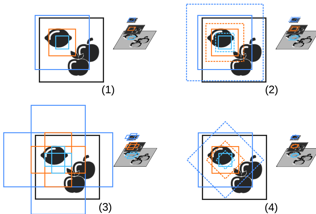
Schema for anchors in the feature map (right) and in the input image (left). (1) Anchors are created on the feature maps of different levels, e.g., the ones drawn (in light blue, orange, and dark blue). (2) Anchors of different sizes are created setting 'anchor_num_subscales' . (3) Anchors of different shapes are created setting 'anchor_aspect_ratios' . (4) Anchors of different orientations are created setting 'anchor_angles' (only for instance type 'rectangle2' ).
