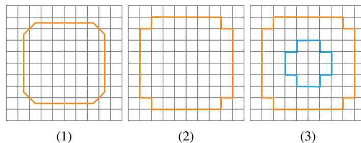
Result for 'center' (1), 'border' (2), and 'border_holes' mode (3).
