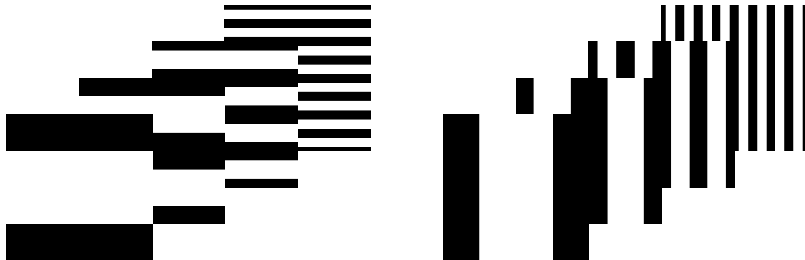
Image series of vertical and horizontal Gray code images as generated by gen_structured_light_pattern . The patterns are typically displayed on the monitor from the coarsest pattern to the finest one while the stripe width is halved at each level.
