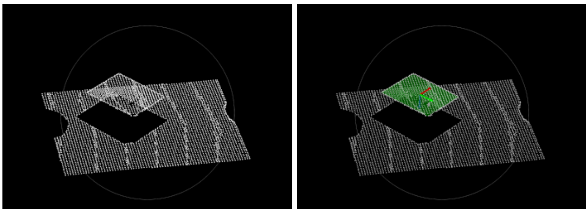
(1) 3D input data (scene), (2) found instance, including a gripping point.
